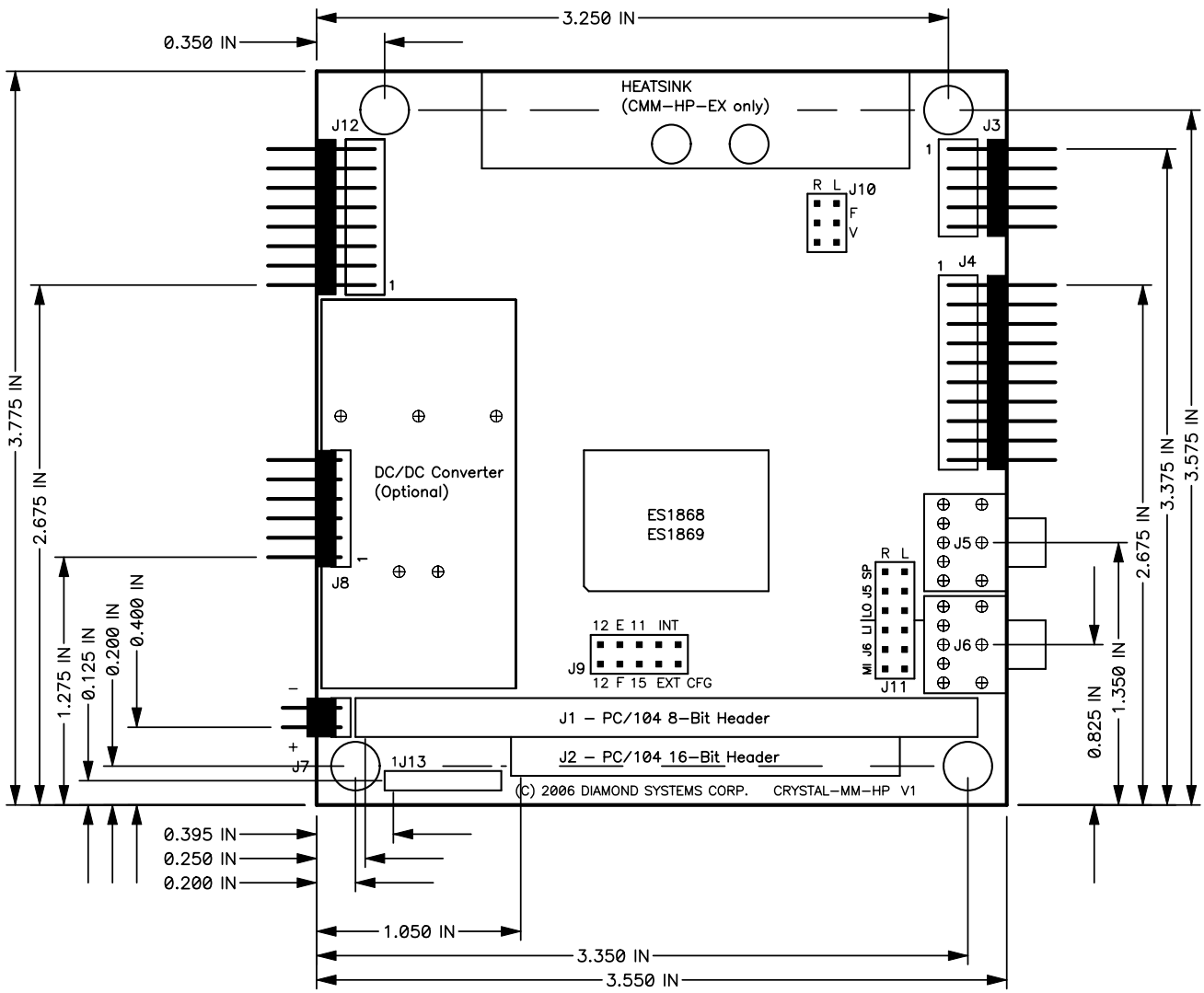
CMM-HP Mechanical Drawing
